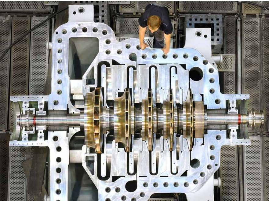
Cross-section of an RH71 compressor from Everllence
