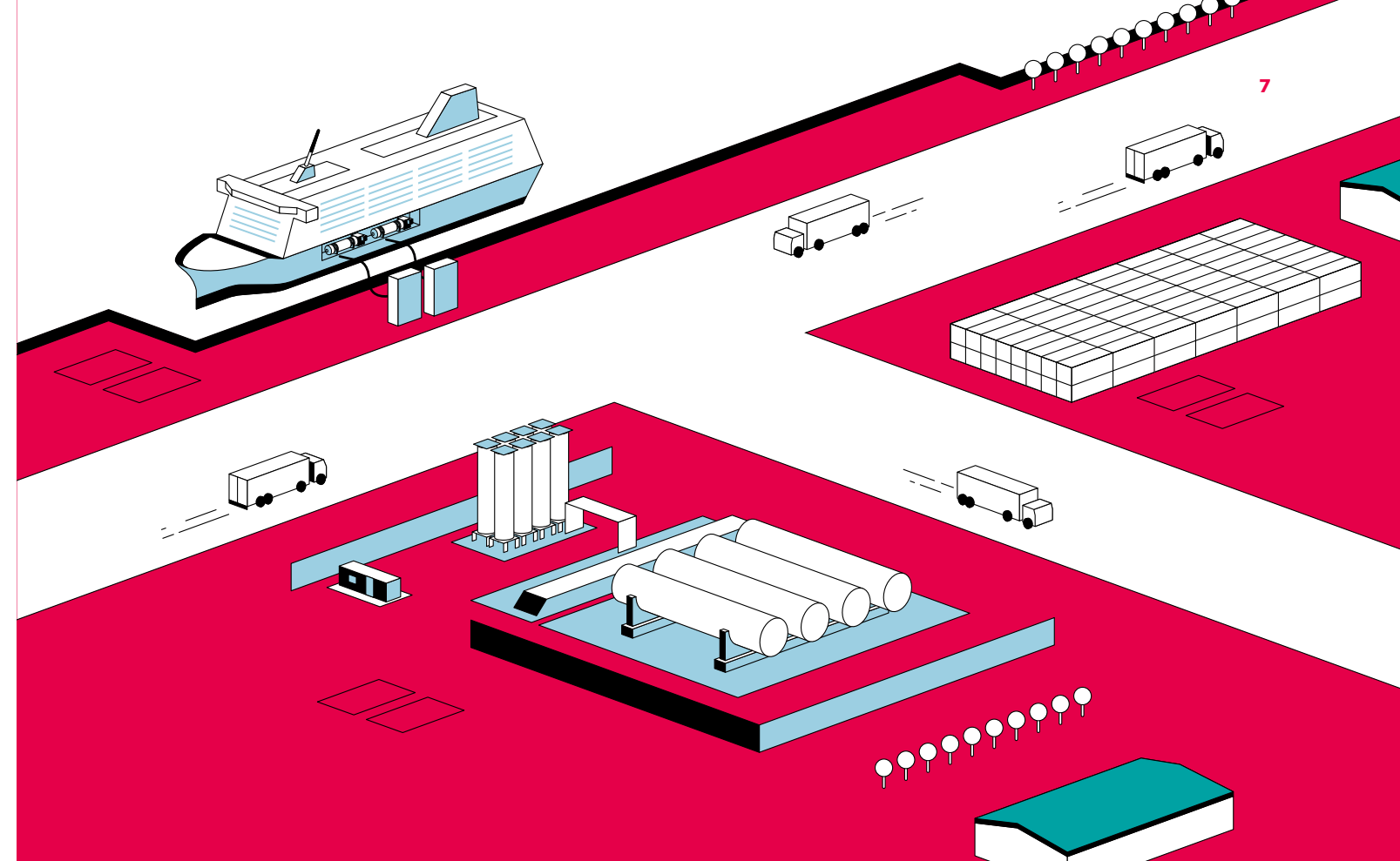
Fig.1 Low pressure fuel gas supply system (LP FGSS) based on LNG supply and bunkering systems
