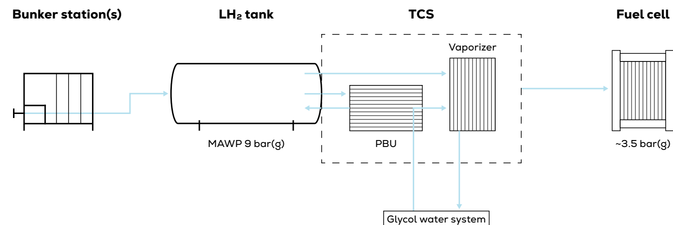
Fig. 2 LH 2 FGSS with PBU
